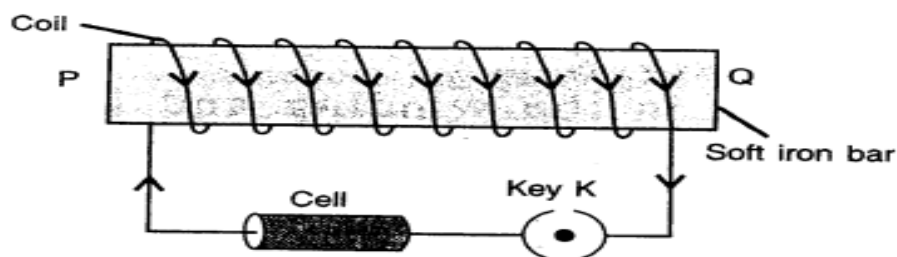
Making a bar electromagnet
